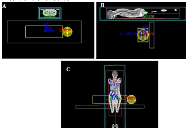
Figure 1. Three views of the geometry setup with the ICRP phantom in the green box as medical personnel and the geometric phantom in the yellow box as the patient; (a) top view; (b) lateral view; (c) front view.
