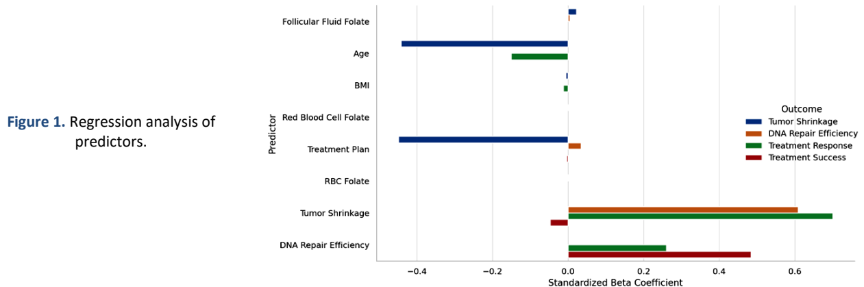
Regression Analysis of Predictors for Radiotherapy Outcomes
