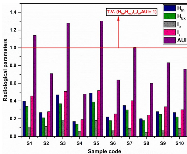
Figure 3. Variations in radiological parameters ( H_{in} , H_{ex} , I_a , I_y , and AUI) for each soil sample, along with their recommended safety threshold values (T.V).
