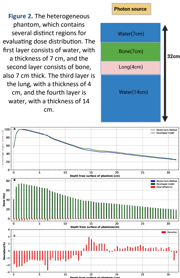
Figure 3. Illustration the dose distribution along the center of the heterogeneous phantom. (a) Percent Dose Depth (PDD) curves were generated using Monte Carlo simulations and predicted by the developed model. (b) The actual values of the dose distribution were obtained using both methods, along with the differences in dose distribution values. (c) The dose deviation was determined using the Monte Carlo simulation and predicted by the developed model.
