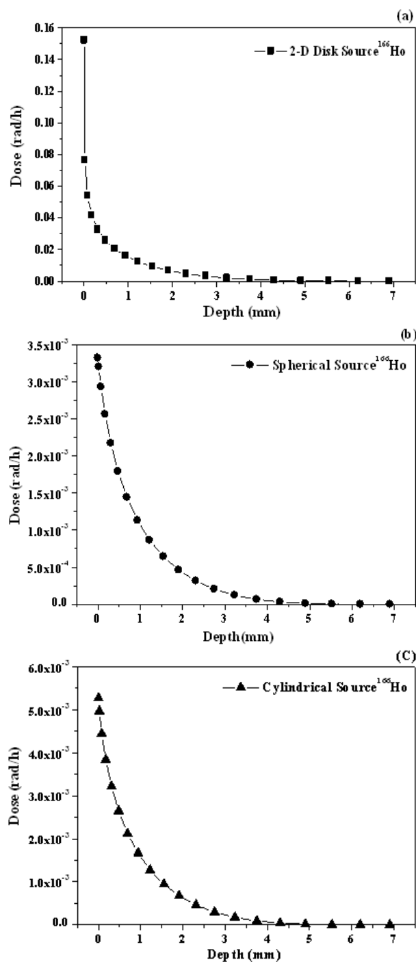
Figure 2. The absorbed depth dose variation for three kind of ^{166}\text{Ho} source geometry with activity 1\mu\text{Ci} (a) 2-D disk, (b) Spherical and (c) Cylindrical.
