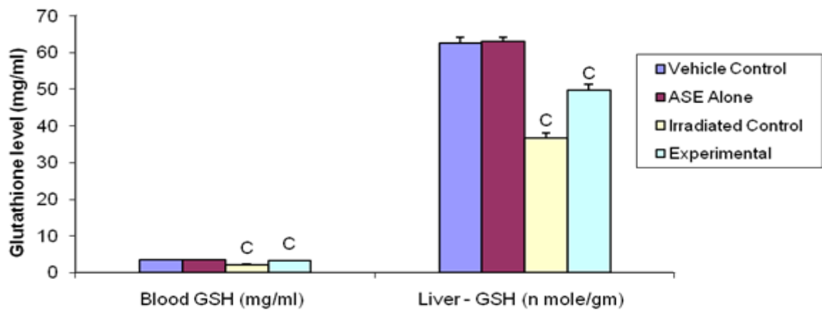
Figure 2. Reduced glutathione (GSH) level in blood and liver of Swiss albino mice after exposure to 7.5 Gy gamma rays with (Experimental) or without (Control) Alstonia scholaris extract (ASE).
