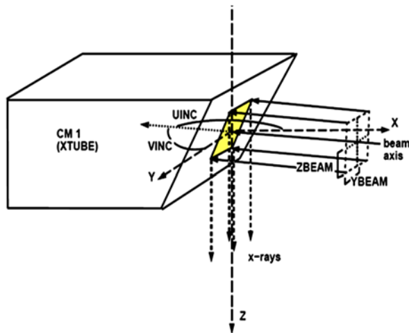
Figure 2. X-ray source used in simulation (Rectangular type source with focal spot size of 8×8mm 2 ).
