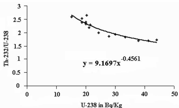
Figure 3. 232 Th/ 238 U activity ratio versus concentration of 238 U in soil.
