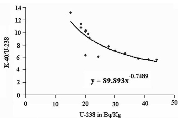
Figure 4. 40 K/ 238 U activity ratio versus concentration of 238 U in soil.
