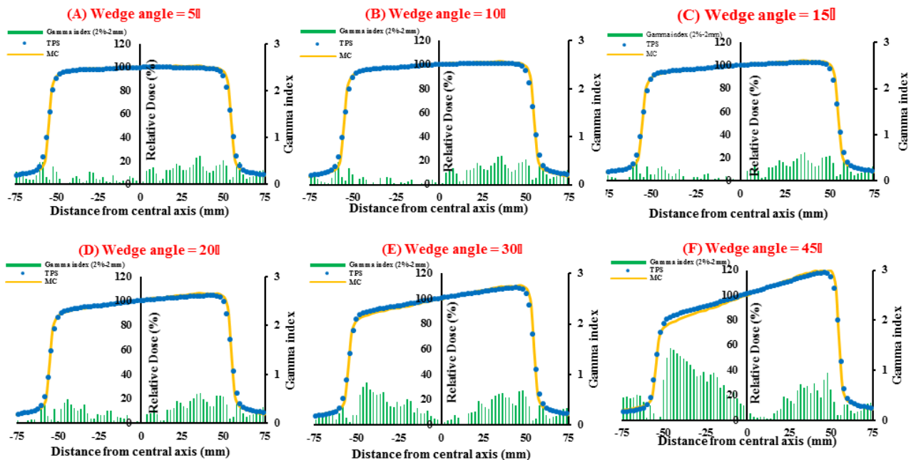
Figure 3. TPS and MC's effective wedge dose profiles comparison beside the gamma index results with 2%-2mm criteria for 10 \times 10 cm 2 at 10 cm depth, 5° (A), 10° (B), 15° (C), 20° (D), 30° (E), 45° (F).
