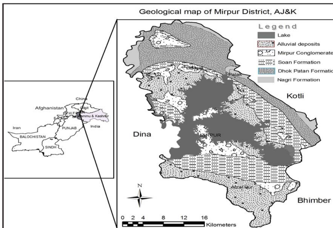
Figure 1. Geological map of Mirpur, Azad Kashmir
