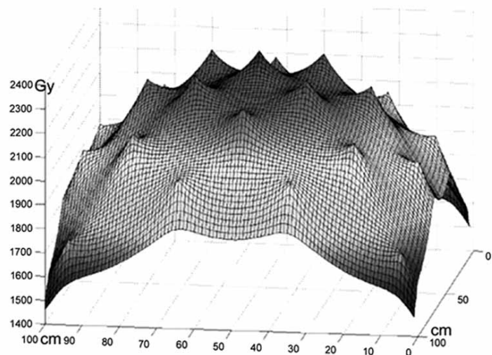
Figure 2. Dose distribution graph of 25 linear sources in 1 m 2 area.
