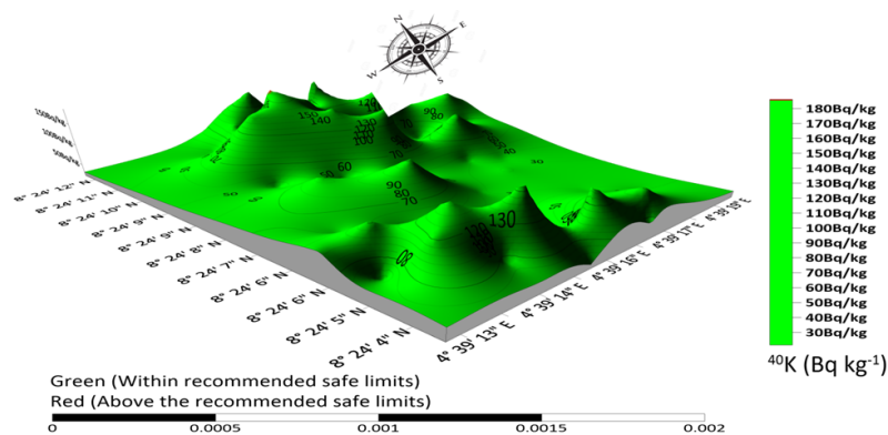
Figure 2. Isopotassium map of the laterite mining field.
