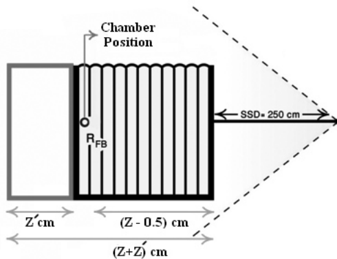
Figure 4. Feature of determination of backscatter correction factor.
