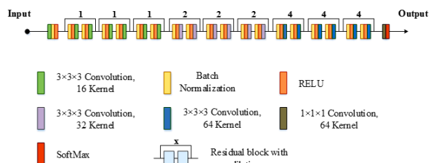
Figure 2. The architecture of ResNet model.
