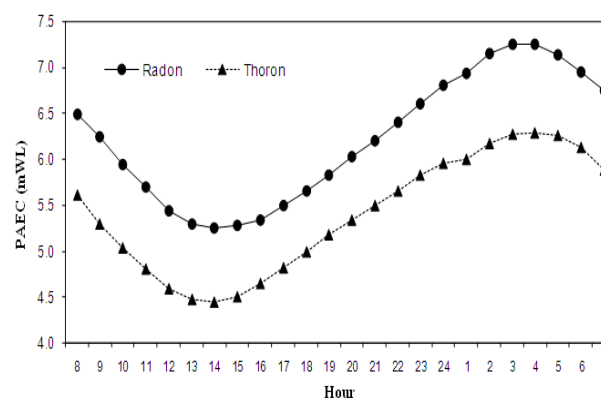
Figure 3. Diurnal variations in radon and thoron progeny in dwellings of Gudalur.
