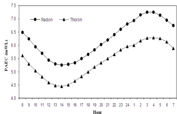
Figure 3. Diurnal variations in radon and thoron progeny in dwellings of Gudalure.
