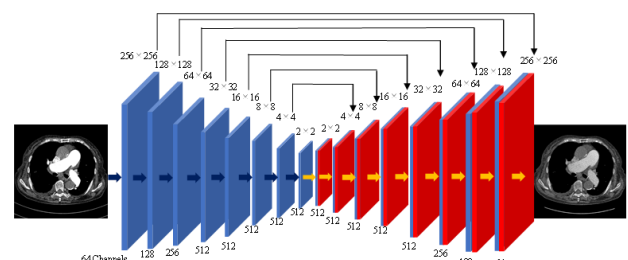
Figure 2. Pix2pix model comprises generator U-Net.
